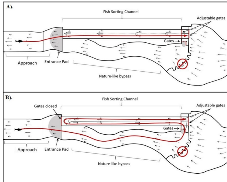
Figure 4. Flow direction and fish movement during (A) normal operating conditions and (B) operating conditions where flow is directed down one side of the fish sorting channel, up the other, and then directed out into the upstream end of the bypass channel.
